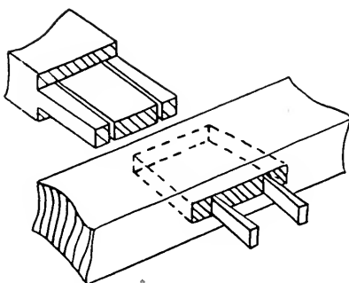
WEDGED MORTISE &amp; TENON
